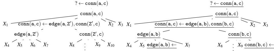
Fig. 3. The infinite rewriting trees T and T' for the program P_4 of Example 4.3, the clause \text{conn}(a, c) , and the substitutions id and \{Z' \mapsto b\} , respectively. T offers no proof that P_4 logically entails \text{conn}(a, c) , but the underlined steps in T' comprise precisely such a proof. The figure also illustrates a transition from T to T' relative to variable X_6 .
